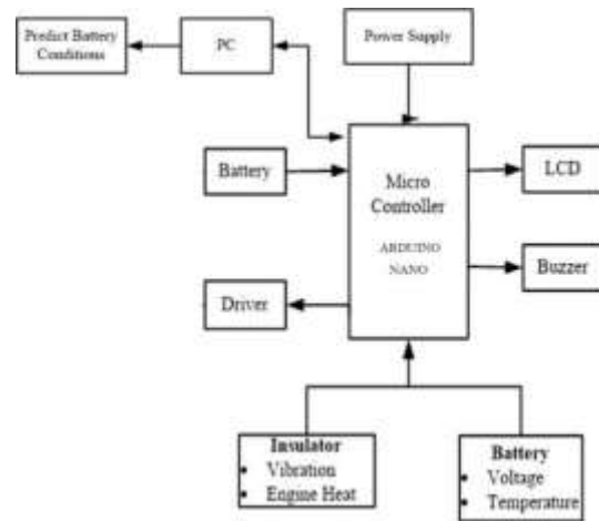
BLOCK DIAGRAM
